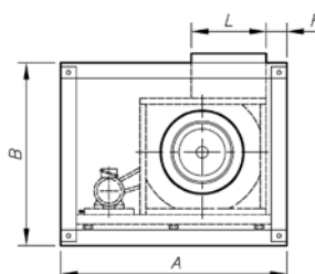
Vertical impulsion on request (V) LG-0
